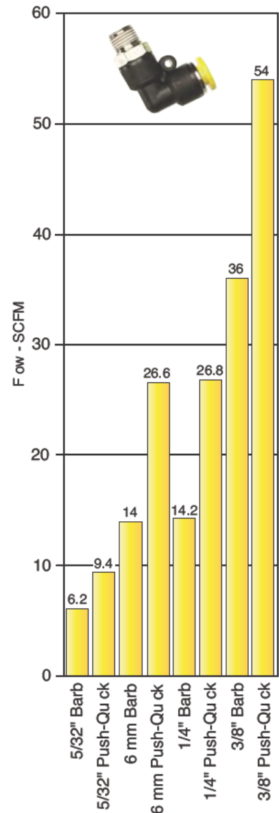
Barb vs Push Quick Fittings Flow Comparison @ 100 psig
