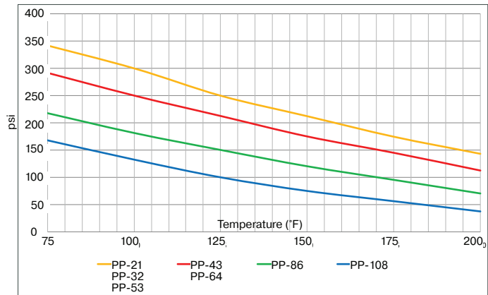
Polypropylene Tubing (Series PP & PPB) Maximum Working Pressure (psi)
