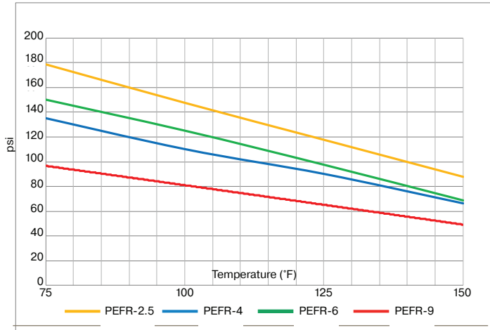
Flame Resistant Polyethylene Tubing (Series PEFR) Maximum Working Pressure (psig)
