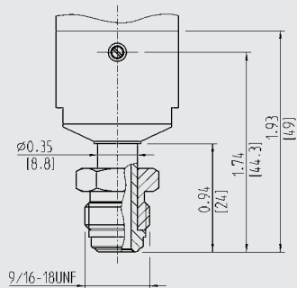
1/4" Swivel Male Face Seal
