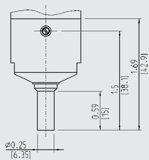
1/4" Weld Stub
