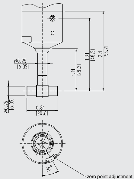
1/4" T-Connector, Weld Stub
