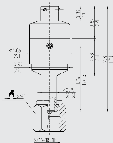
1/4" Swivel Male Face Seal
